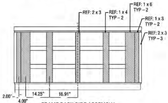
FRAME BACK SIDE ASSEMBLY
